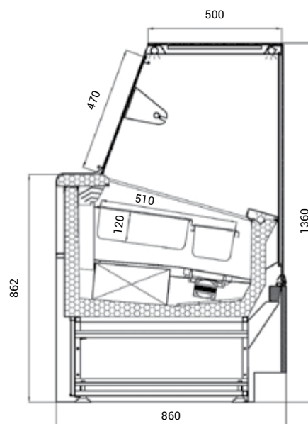
bokorys Raffaello Ice
