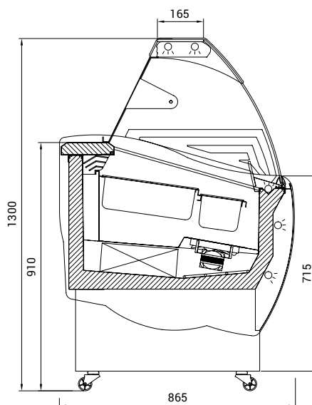
bokorys Cornetti
