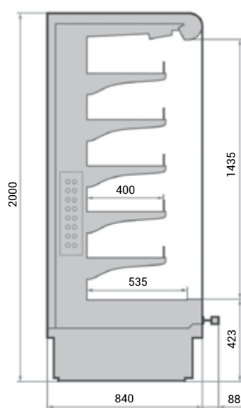
bokorys Scorpion 04
