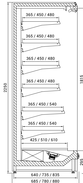
bokorys Praga Plus
